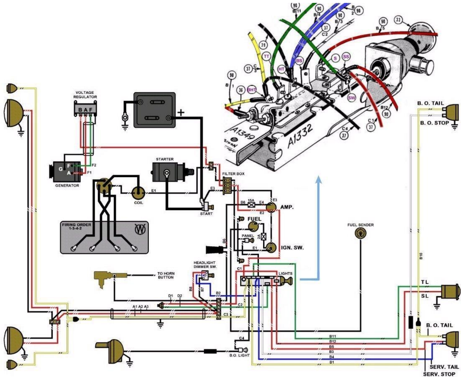
PUSH PULL SWITCH MB / GPW WIRING DIAGRAM
